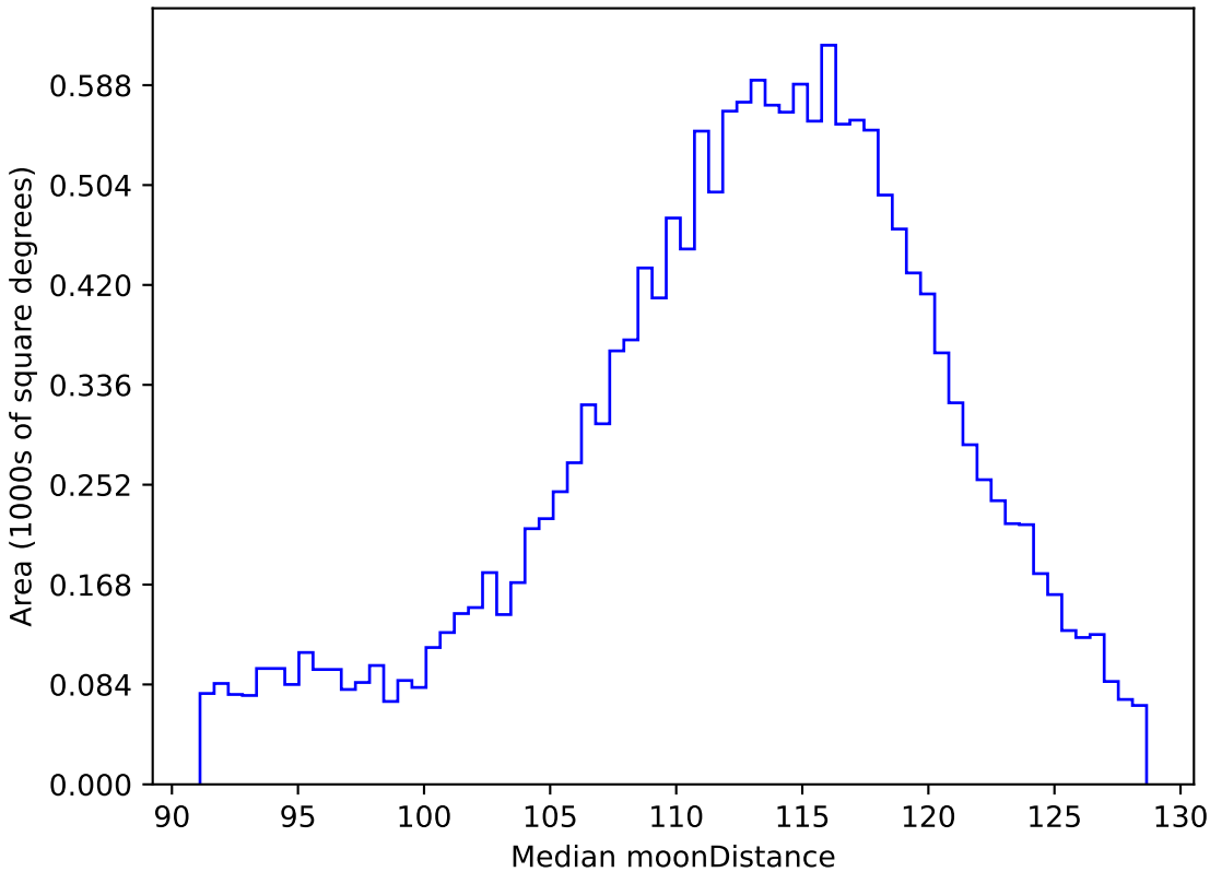
ddf_loaded_fl8_v3.4_10yrs WFD r band: Median moonDistance
