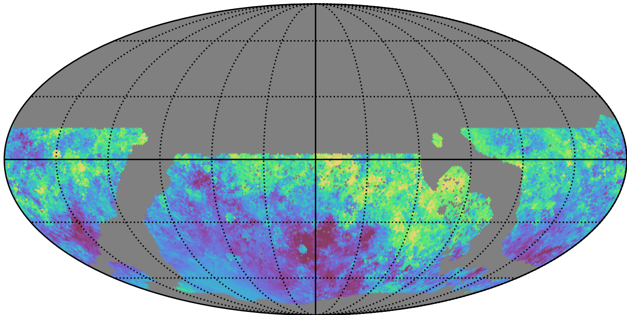
ddf_loaded_fl8_v3.4_10yrs WFD i band: Median moonDistance
