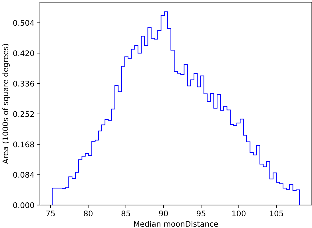
ddf_loaded_fl8_v3.4_10yrs WFD i band: Median moonDistance
