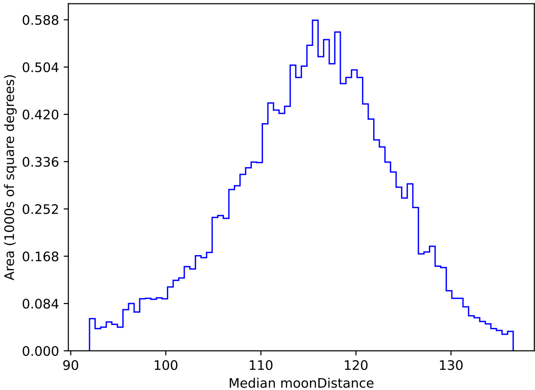
ddf_loaded_fl8_v3.4_10yrs WFD g band: Median moonDistance
