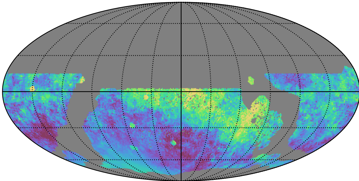
ddf_loaded_fl8_v3.4_10yrs WFD all bands: Median moonDistance
