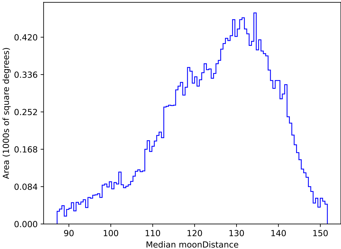
ddf_loaded_fl8_v3.4_10yrs All sky u band: Median moonDistance
