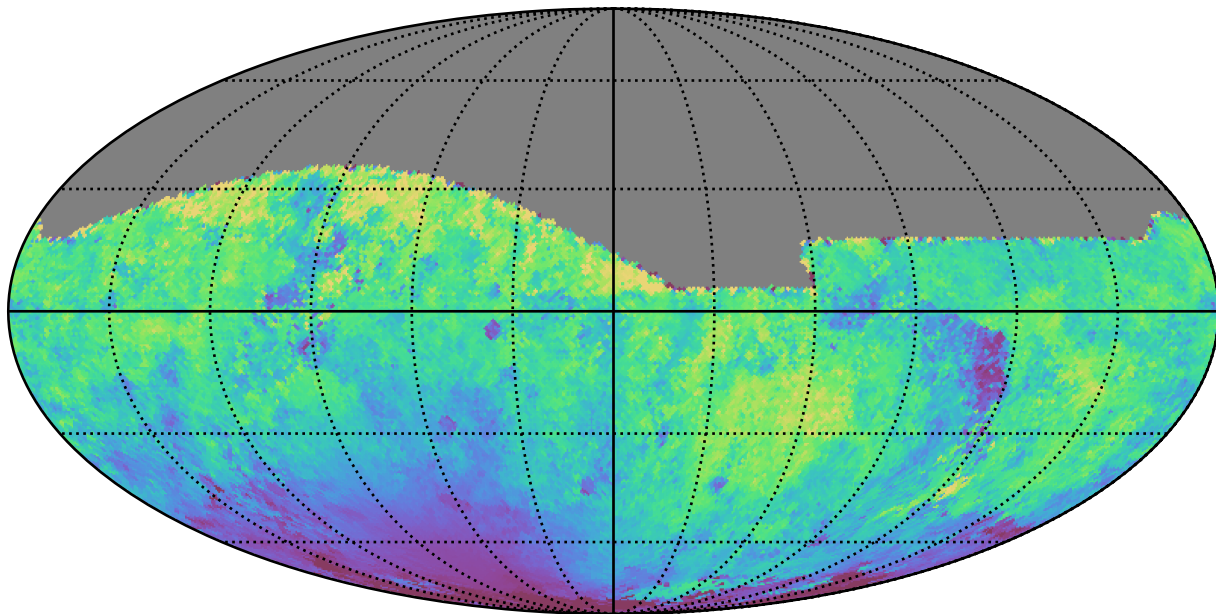
ddf_loaded_fl8_v3.4_10yrs All sky r band: Median moonDistance
