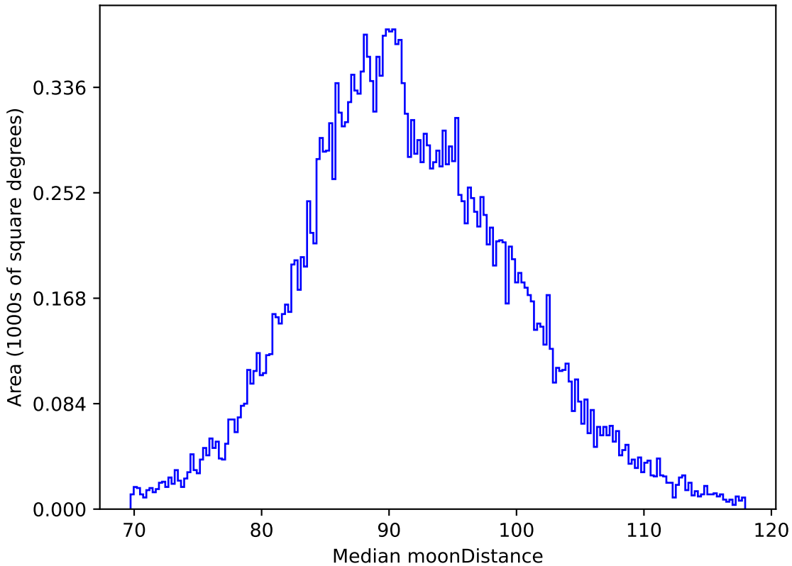
ddf_loaded_fl8_v3.4_10yrs All sky i band: Median moonDistance
