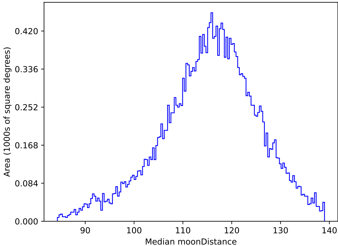
ddf_loaded_fl8_v3.4_10yrs All sky g band: Median moonDistance
