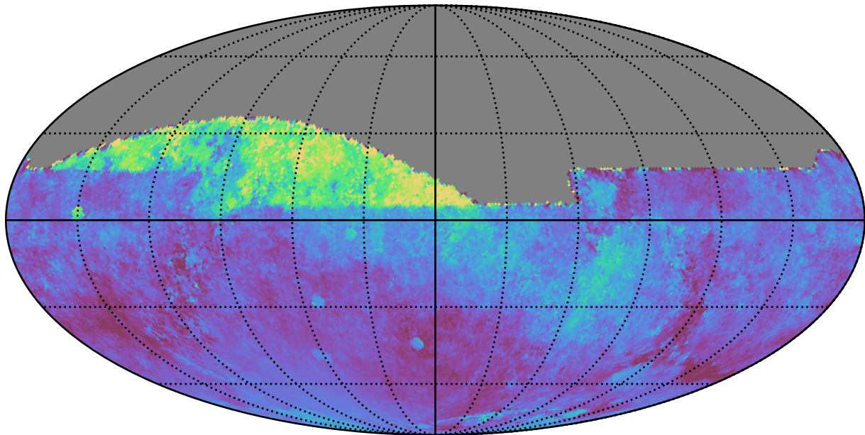
ddf_loaded_fl8_v3.4_10yrs All sky all bands: Median moonDistance
