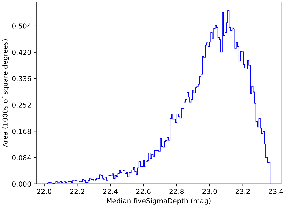
ddf_loaded_fl8_v3.4_10yrs Yr 1 z band: Median fiveSigmaDepth
