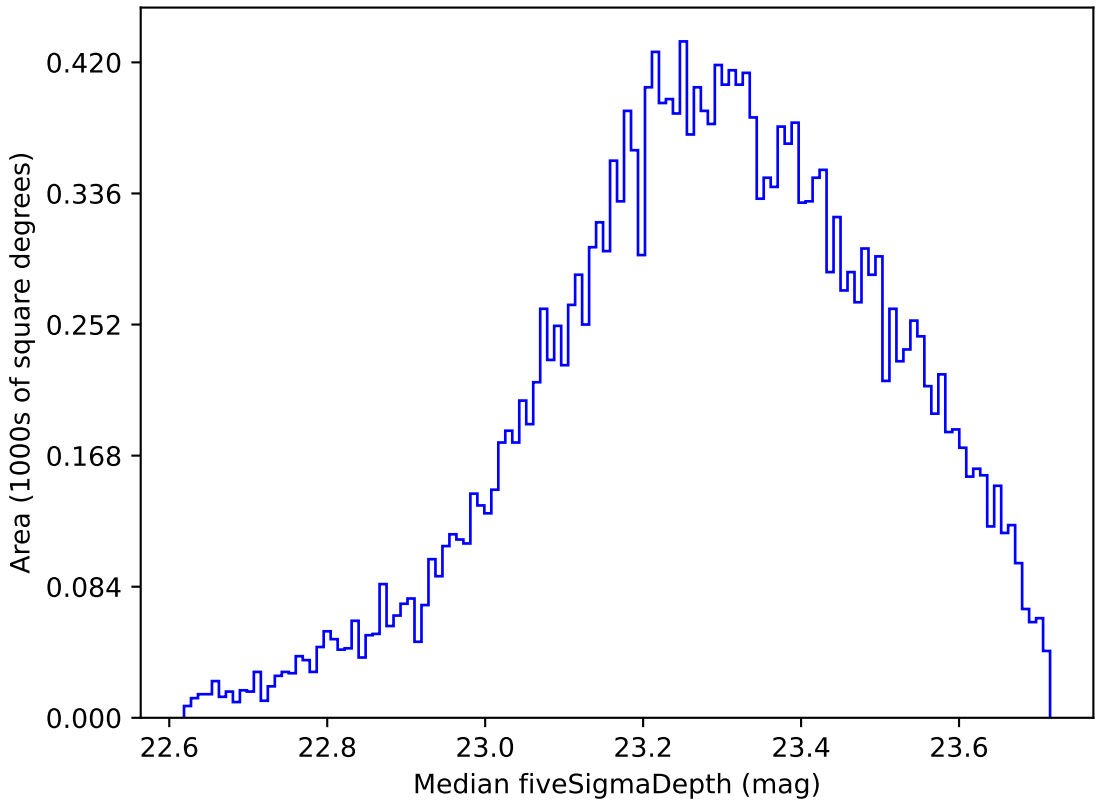
ddf_loaded_fl8_v3.4_10yrs Yr 1 u band: Median fiveSigmaDepth
