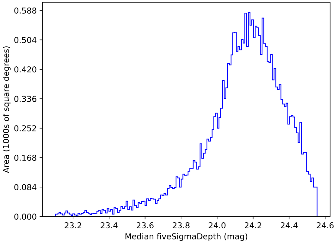
ddf_loaded_fl8_v3.4_10yrs Yr 1 r band: Median fiveSigmaDepth
