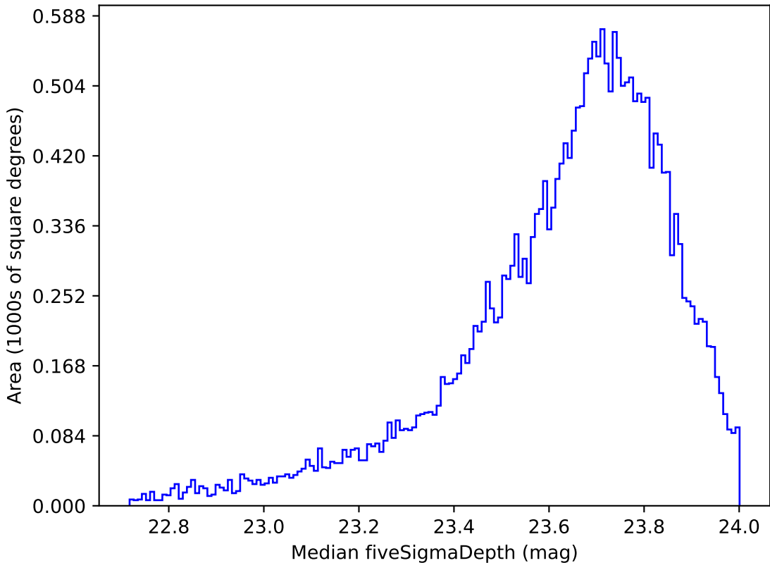
ddf_loaded_fl8_v3.4_10yrs Yr 1 i band: Median fiveSigmaDepth
