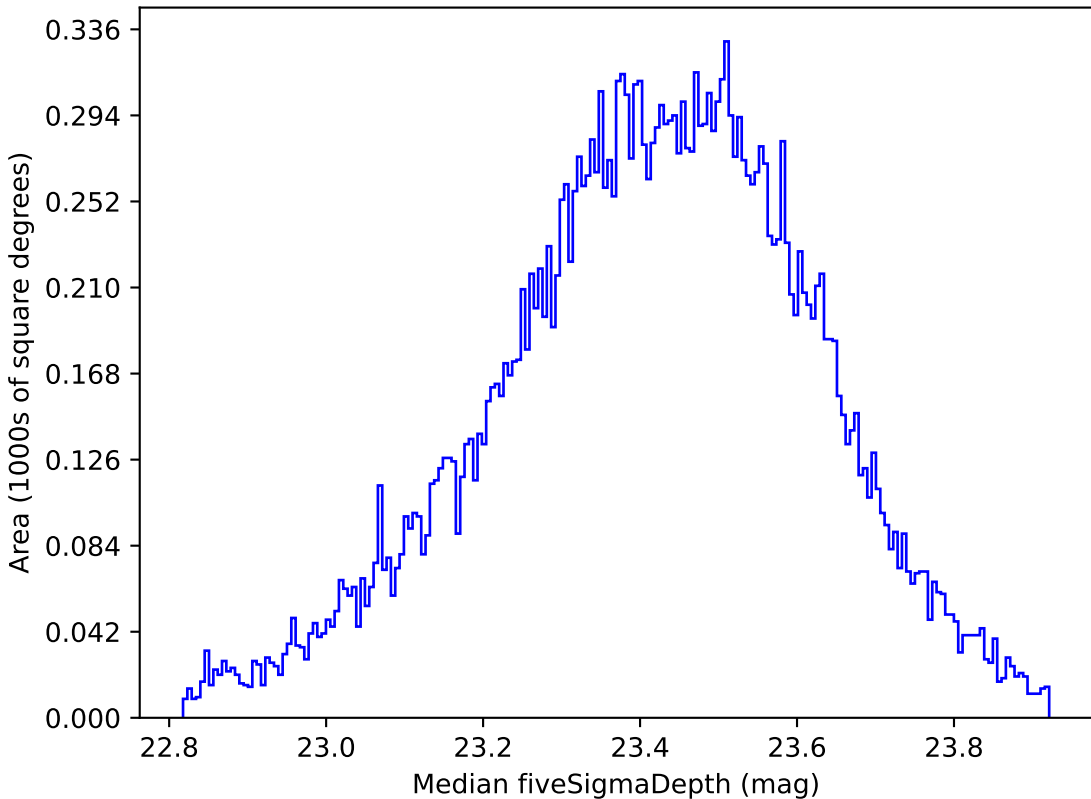
ddf_loaded_fl8_v3.4_10yrs Yr 1 all bands: Median fiveSigmaDepth
