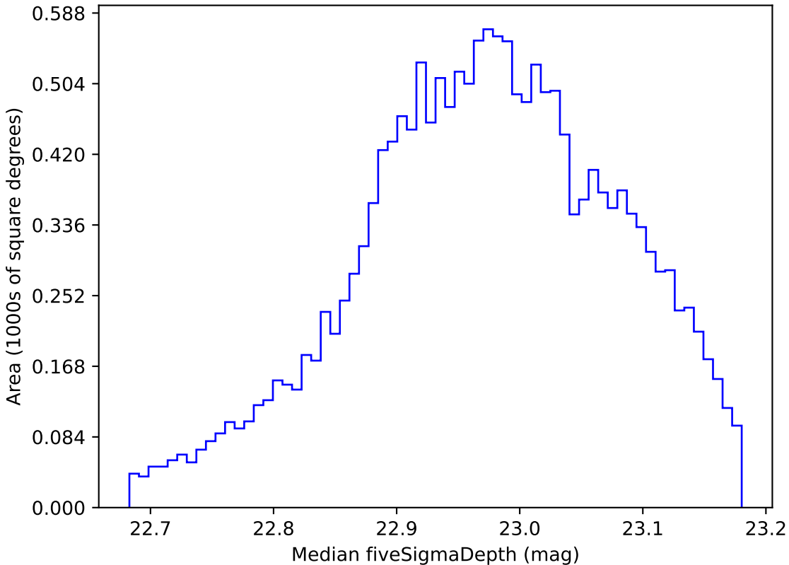
ddf_loaded_fl8_v3.4_10yrs WFD z band: Median fiveSigmaDepth
