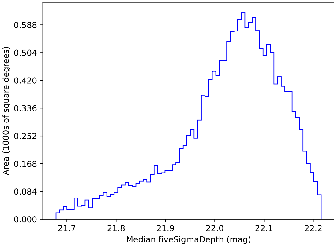
ddf_loaded_fl8_v3.4_10yrs WFD y band: Median fiveSigmaDepth
