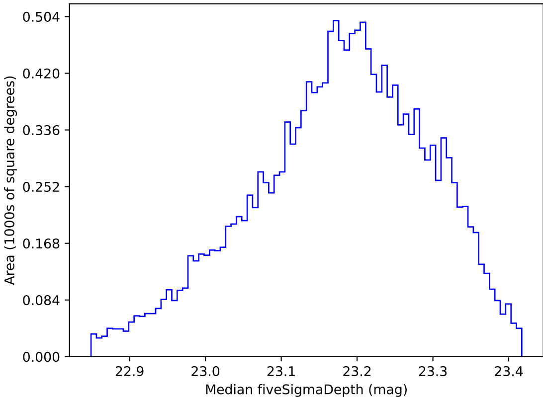
ddf_loaded_fl8_v3.4_10yrs WFD u band: Median fiveSigmaDepth
