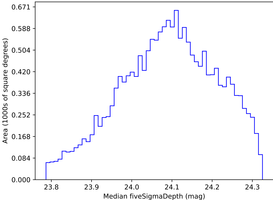
ddf_loaded_fl8_v3.4_10yrs WFD r band: Median fiveSigmaDepth
