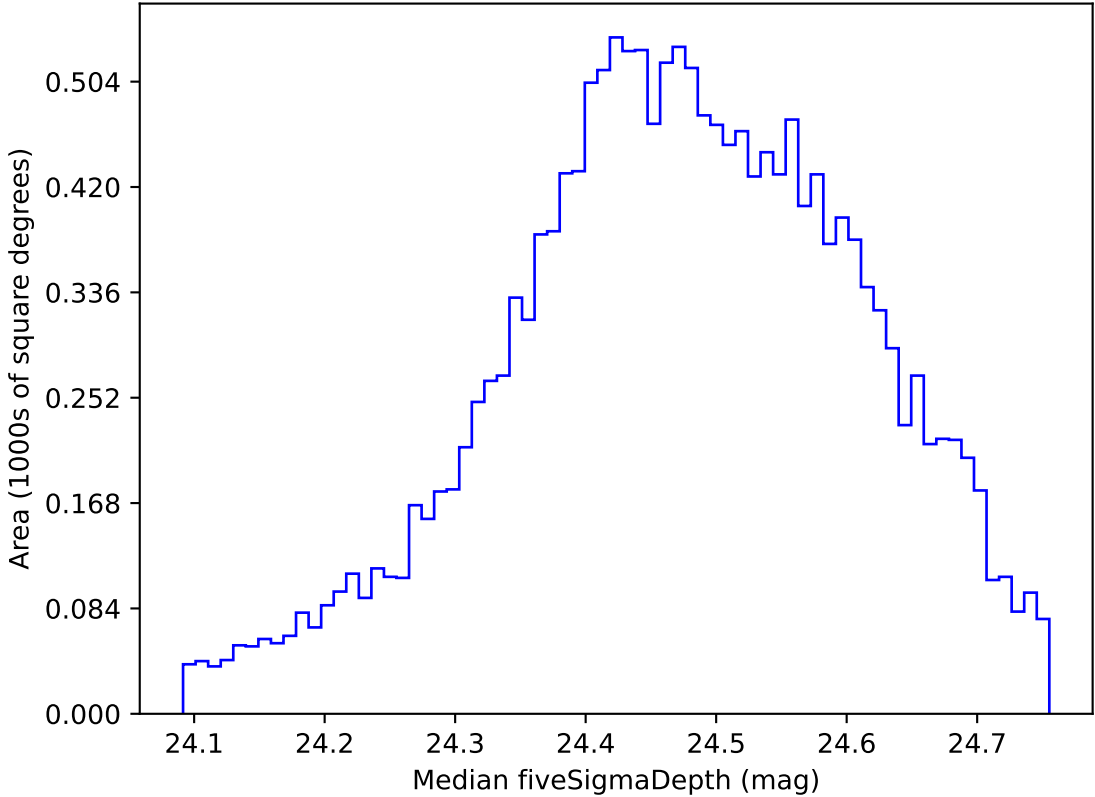
ddf_loaded_fl8_v3.4_10yrs WFD g band: Median fiveSigmaDepth
