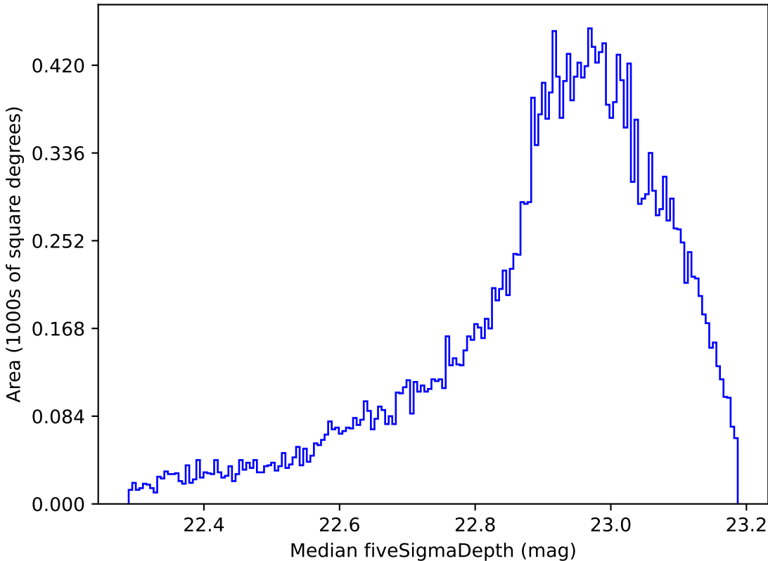
ddf_loaded_fl8_v3.4_10yrs All sky z band: Median fiveSigmaDepth
