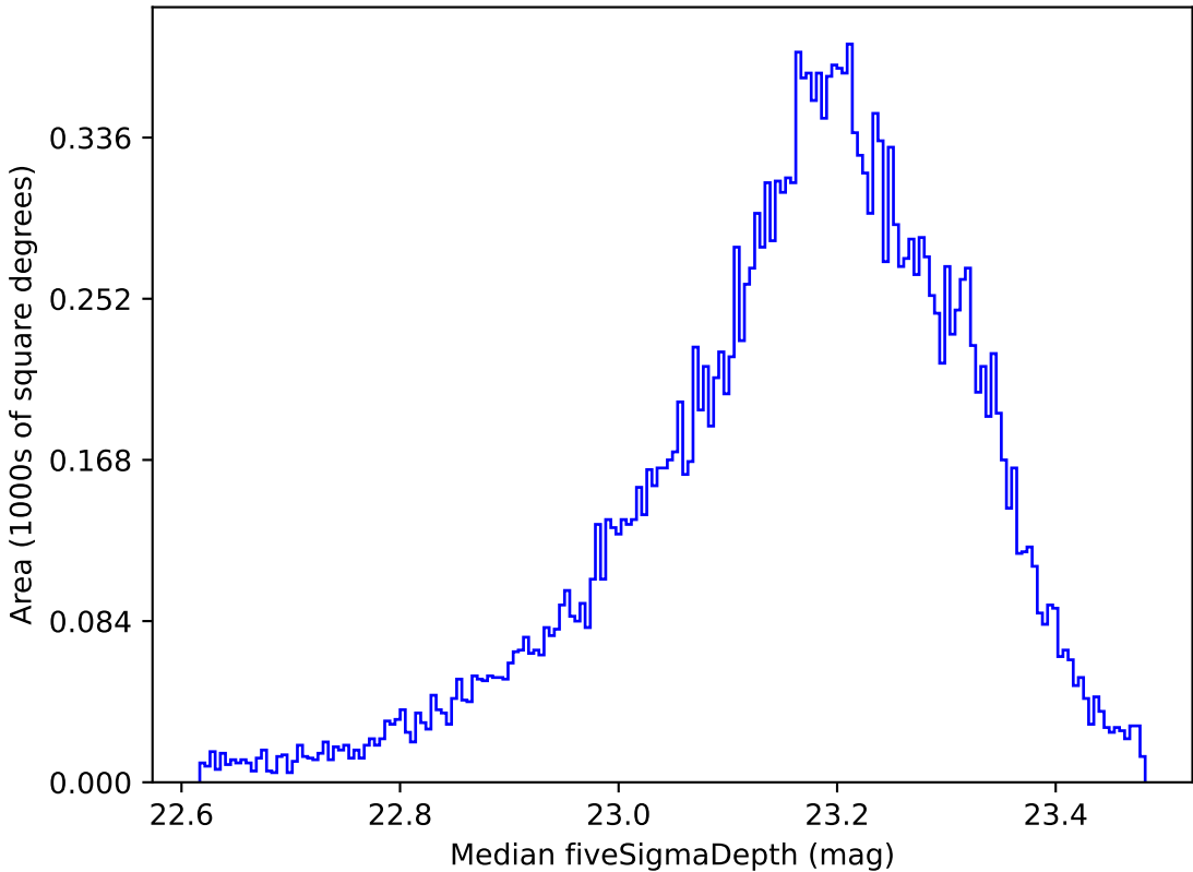
ddf_loaded_fl8_v3.4_10yrs All sky u band: Median fiveSigmaDepth
