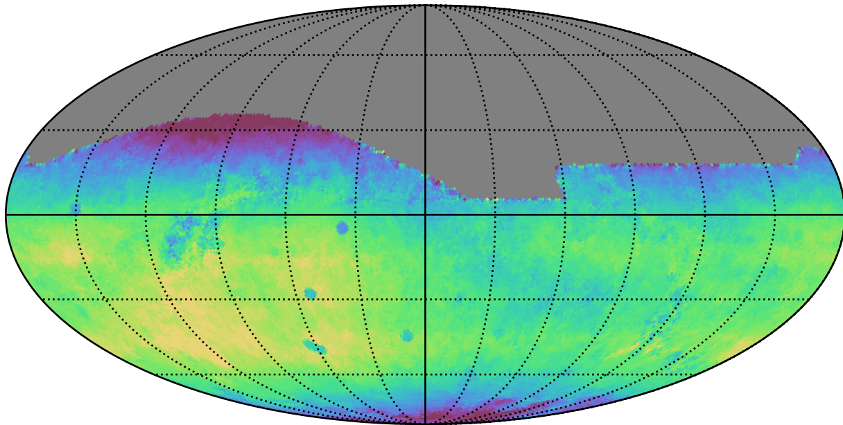
ddf_loaded_fl8_v3.4_10yrs All sky r band: Median fiveSigmaDepth
