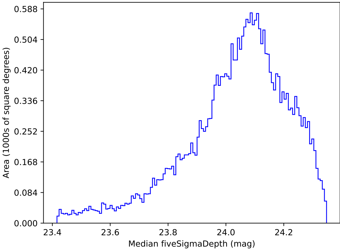
ddf_loaded_fl8_v3.4_10yrs All sky r band: Median fiveSigmaDepth
