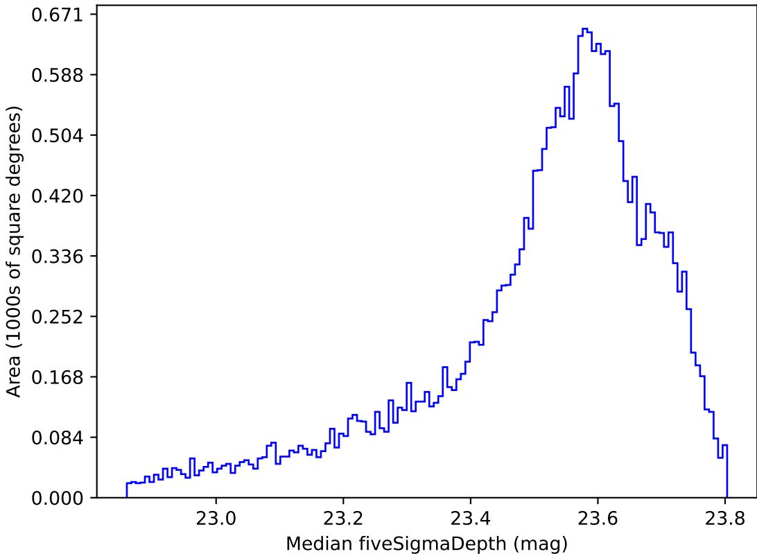
ddf_loaded_fl8_v3.4_10yrs All sky i band: Median fiveSigmaDepth
