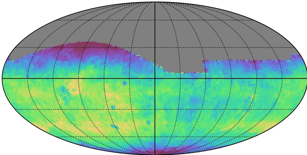
ddf_loaded_fl8_v3.4_10yrs All sky g band: Median fiveSigmaDepth
