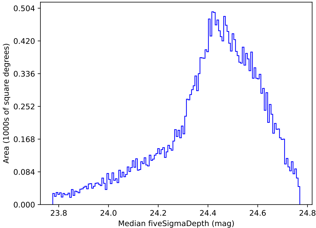
ddf_loaded_fl8_v3.4_10yrs All sky g band: Median fiveSigmaDepth
