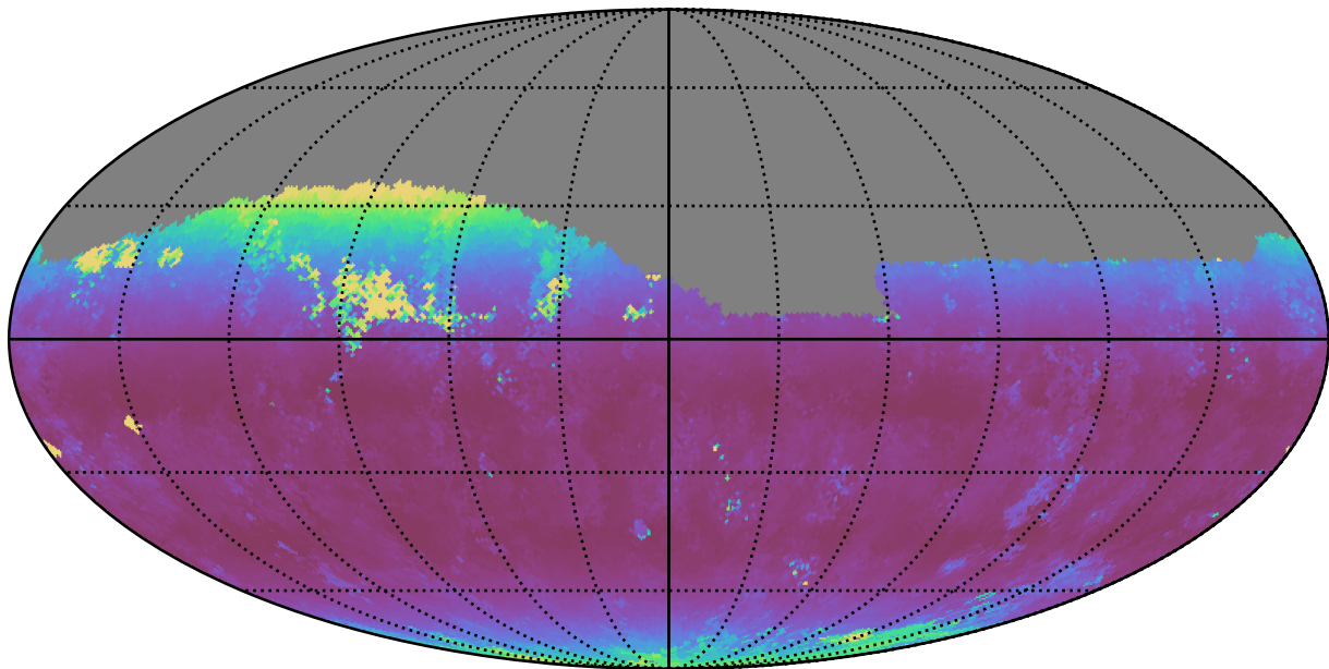
ddf_loaded_fl8_v3.4_10yrs Yr 1 z band: Median airmass
