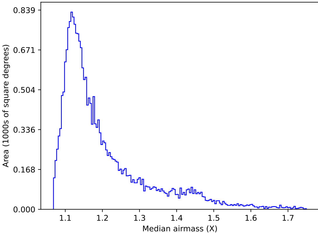
ddf_loaded_fl8_v3.4_10yrs Yr 1 y band: Median airmass
