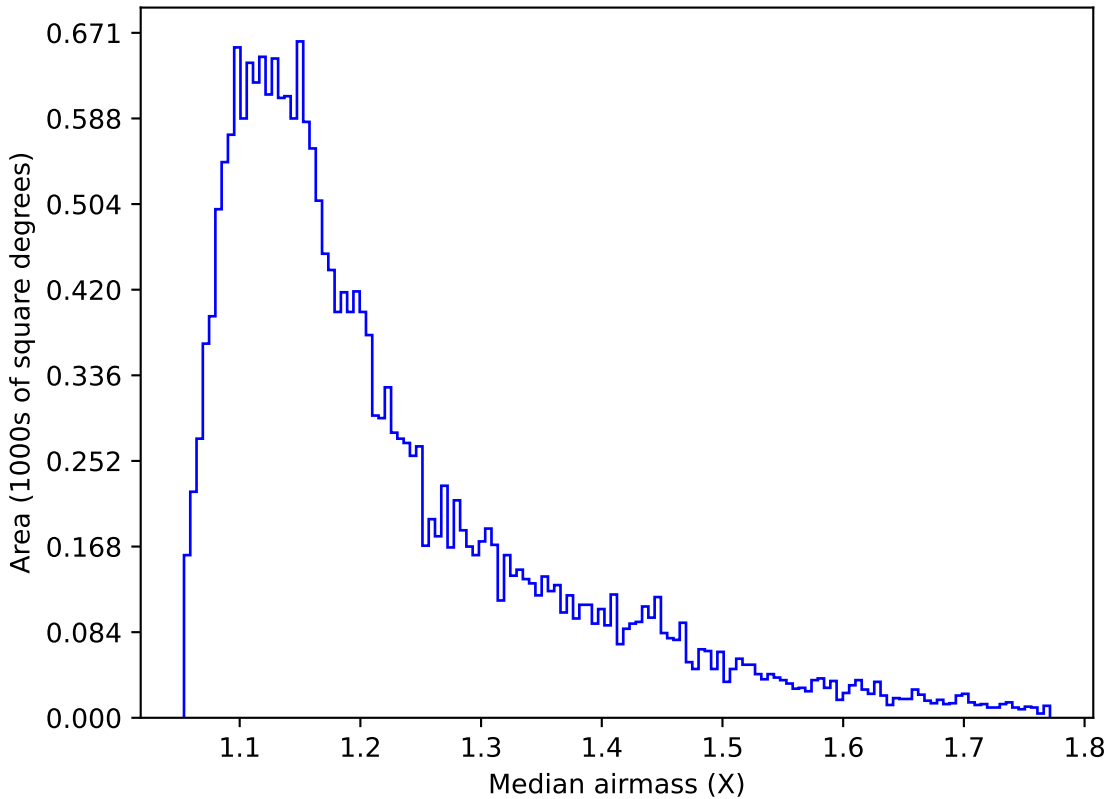
ddf_loaded_fl8_v3.4_10yrs Yr 1 u band: Median airmass
