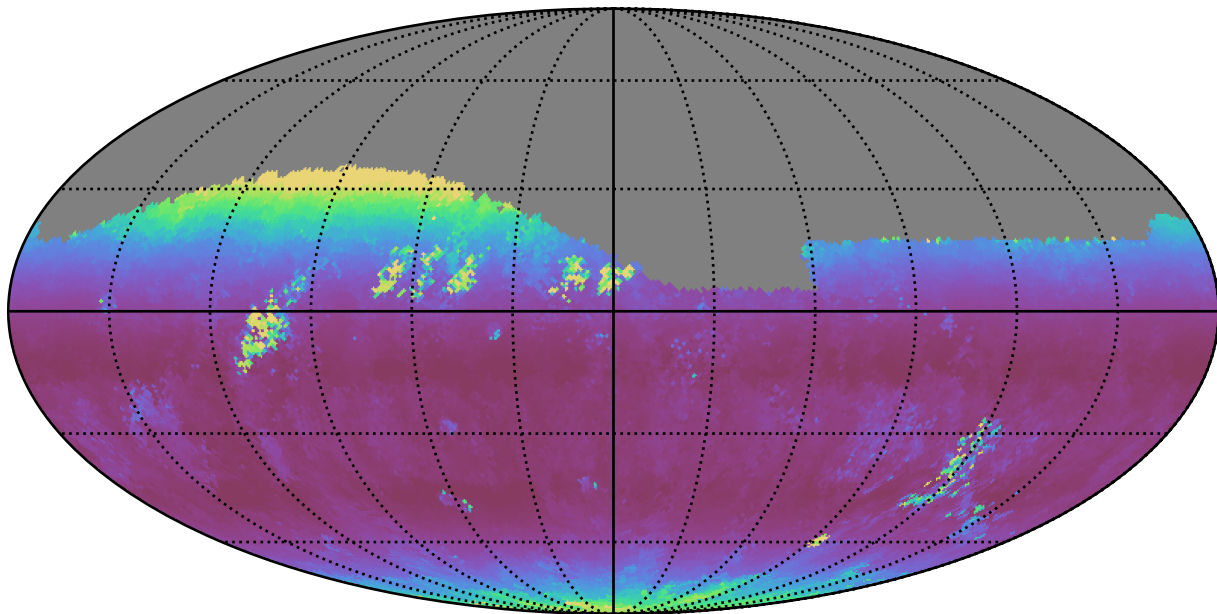
ddf_loaded_fl8_v3.4_10yrs Yr 1 r band: Median airmass
