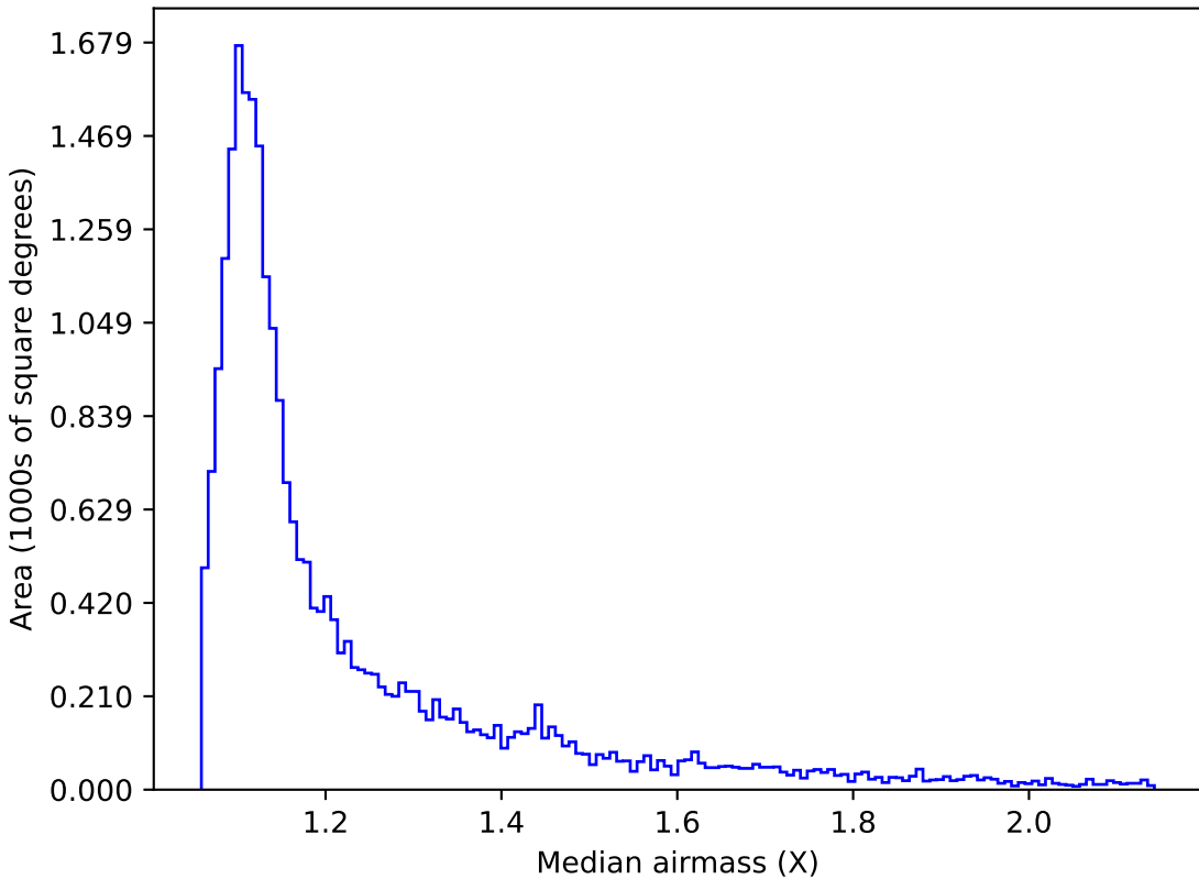
ddf_loaded_fl8_v3.4_10yrs Yr 1 i band: Median airmass
