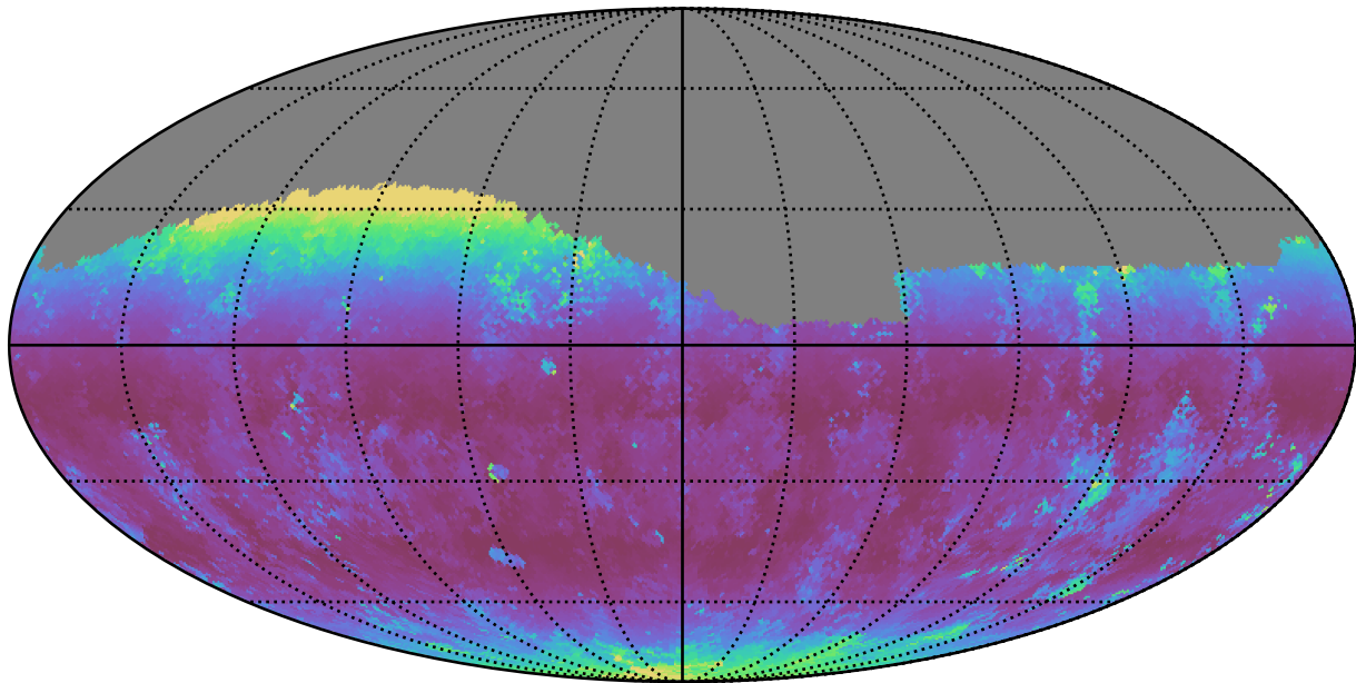
ddf_loaded_fl8_v3.4_10yrs Yr 1 g band: Median airmass
