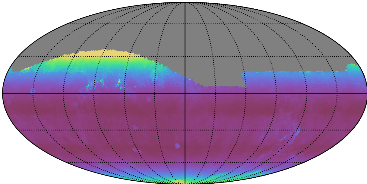
ddf_loaded_fl8_v3.4_10yrs Yr 1 all bands: Median airmass
