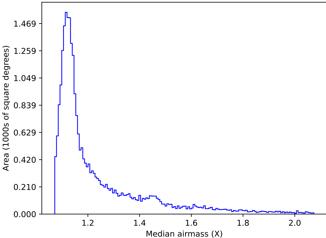
ddf_loaded_fl8_v3.4_10yrs Yr 1 all bands: Median airmass
