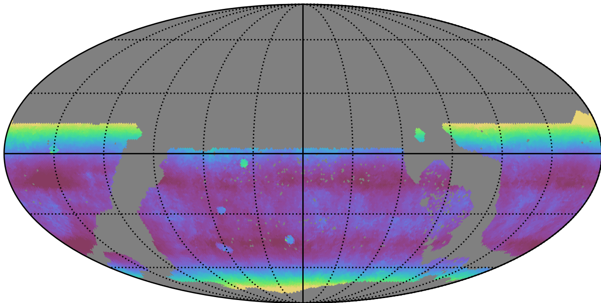
ddf_loaded_fl8_v3.4_10yrs WFD z band: Median airmass
