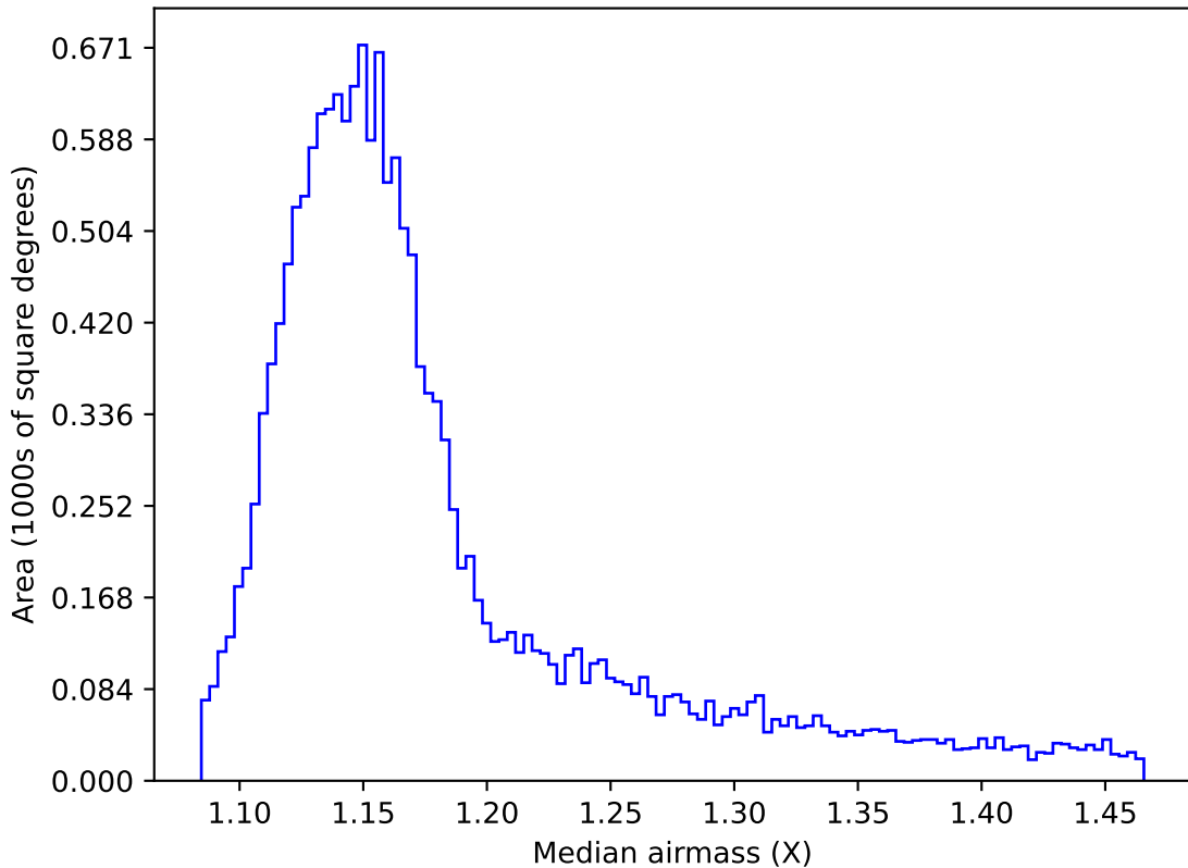
ddf_loaded_fl8_v3.4_10yrs WFD z band: Median airmass
