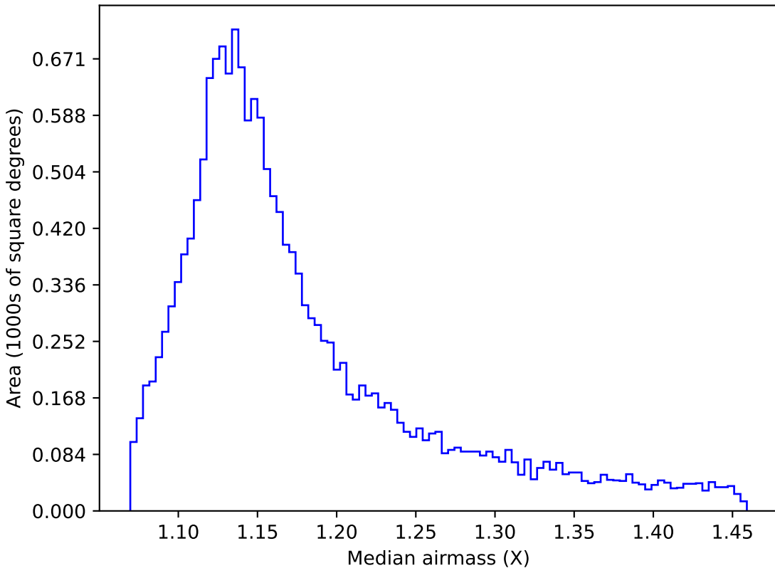
ddf_loaded_fl8_v3.4_10yrs WFD u band: Median airmass
