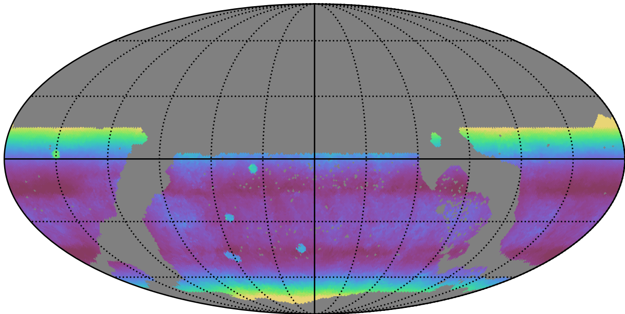
ddf_loaded_fl8_v3.4_10yrs WFD r band: Median airmass
