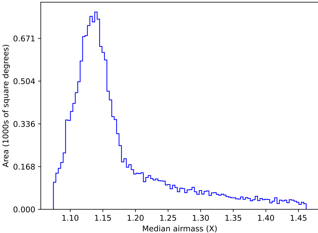
ddf_loaded_fl8_v3.4_10yrs WFD r band: Median airmass
