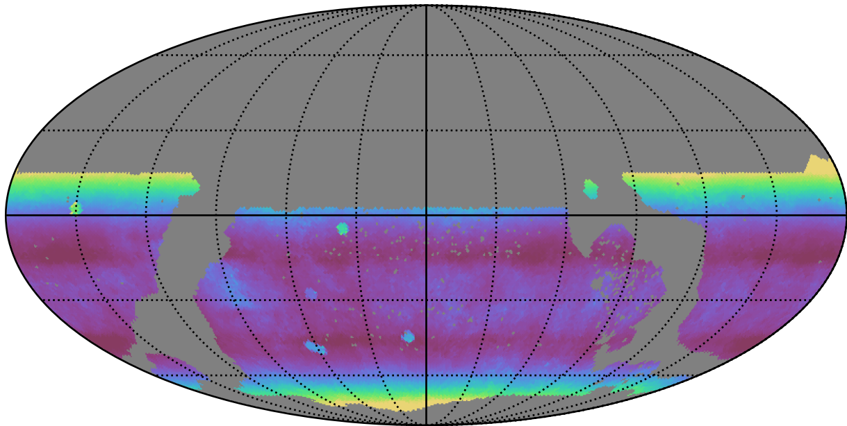
ddf_loaded_fl8_v3.4_10yrs WFD i band: Median airmass
