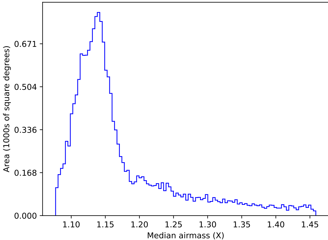
ddf_loaded_fl8_v3.4_10yrs WFD i band: Median airmass
