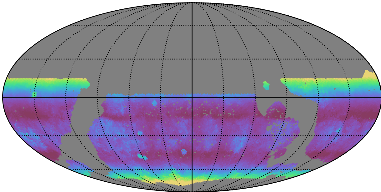
ddf_loaded_fl8_v3.4_10yrs WFD g band: Median airmass
