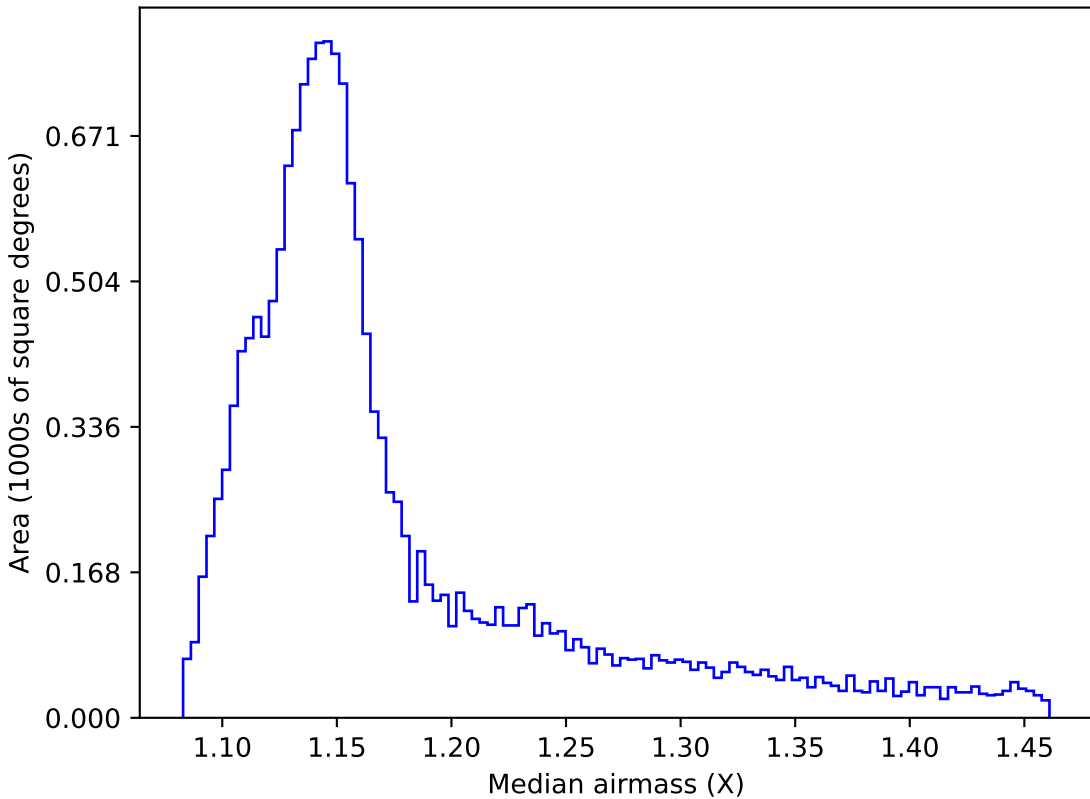
ddf_loaded_fl8_v3.4_10yrs WFD all bands: Median airmass
