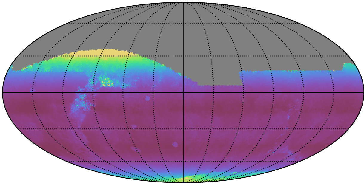
ddf_loaded_fl8_v3.4_10yrs All sky z band: Median airmass
