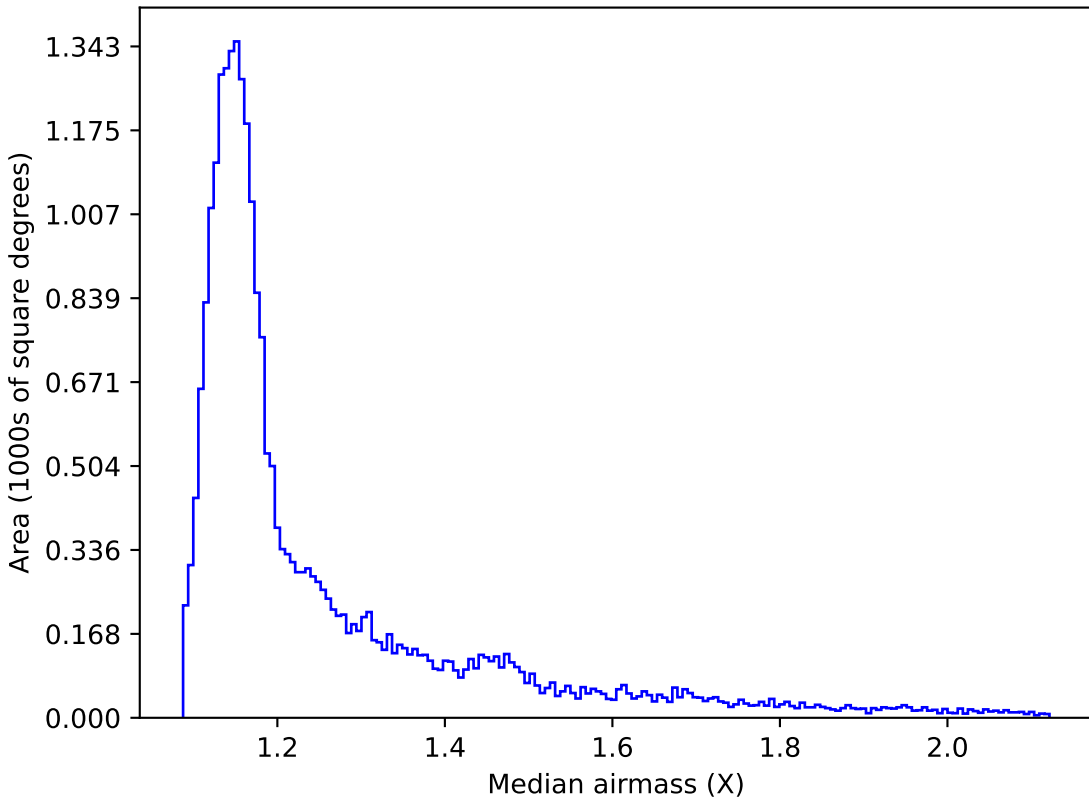
ddf_loaded_fl8_v3.4_10yrs All sky z band: Median airmass
