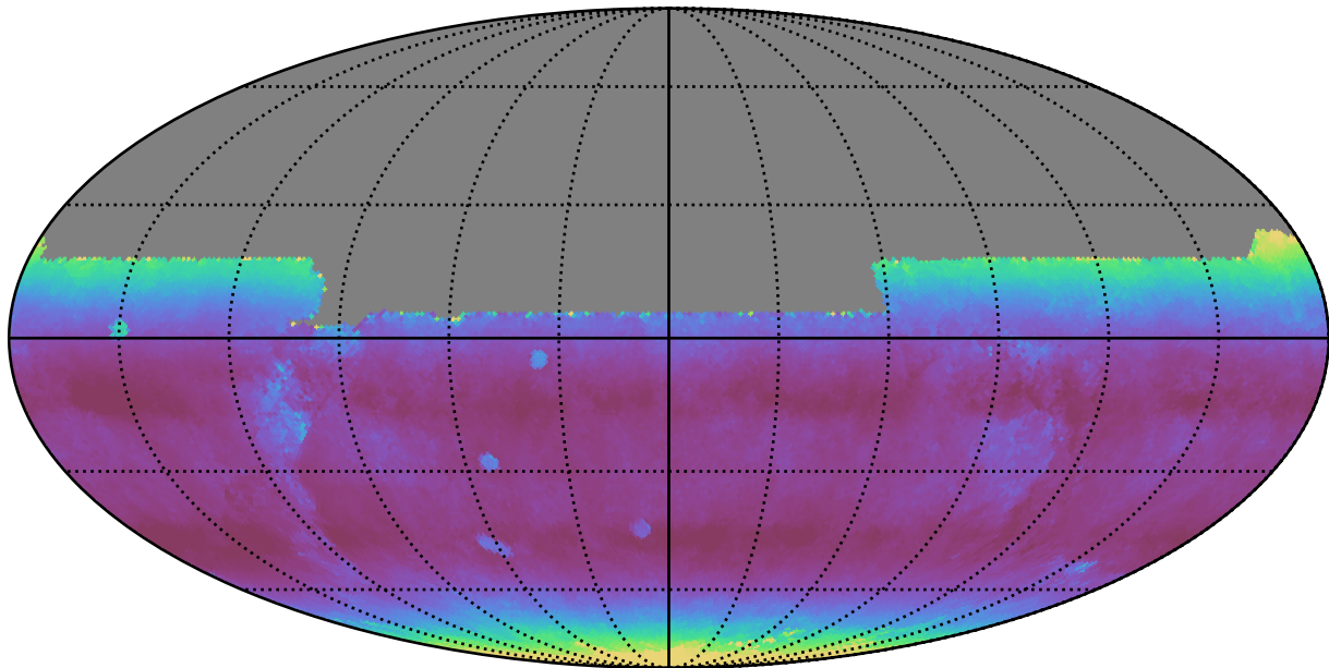
ddf_loaded_fl8_v3.4_10yrs All sky y band: Median airmass
