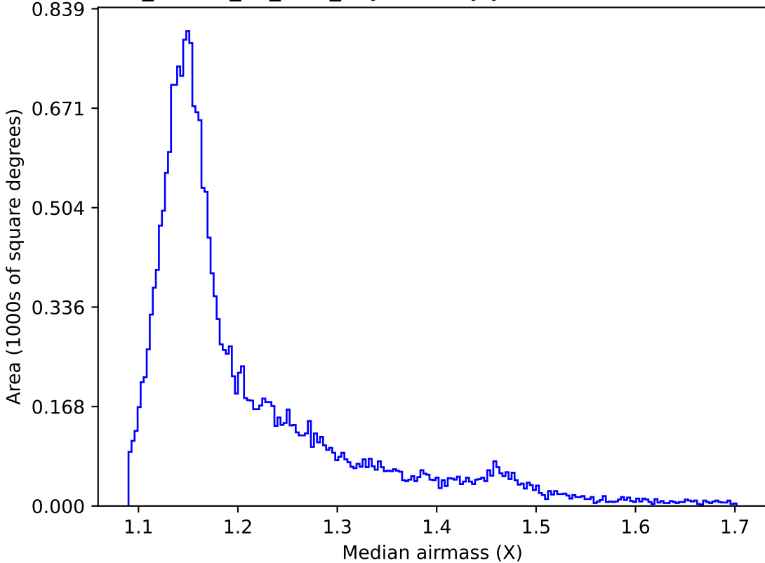
ddf_loaded_fl8_v3.4_10yrs All sky y band: Median airmass
