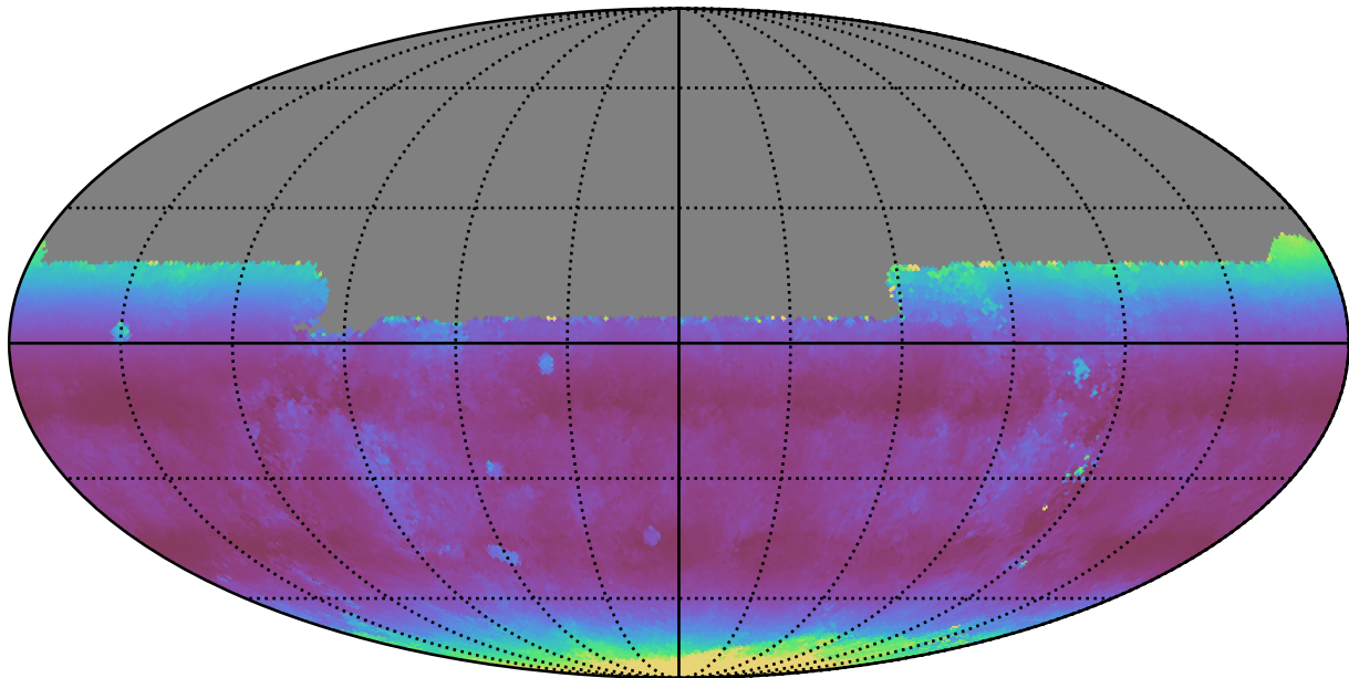
ddf_loaded_fl8_v3.4_10yrs All sky u band: Median airmass
