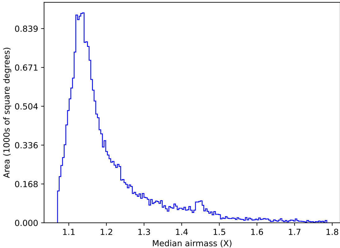
ddf_loaded_fl8_v3.4_10yrs All sky u band: Median airmass
